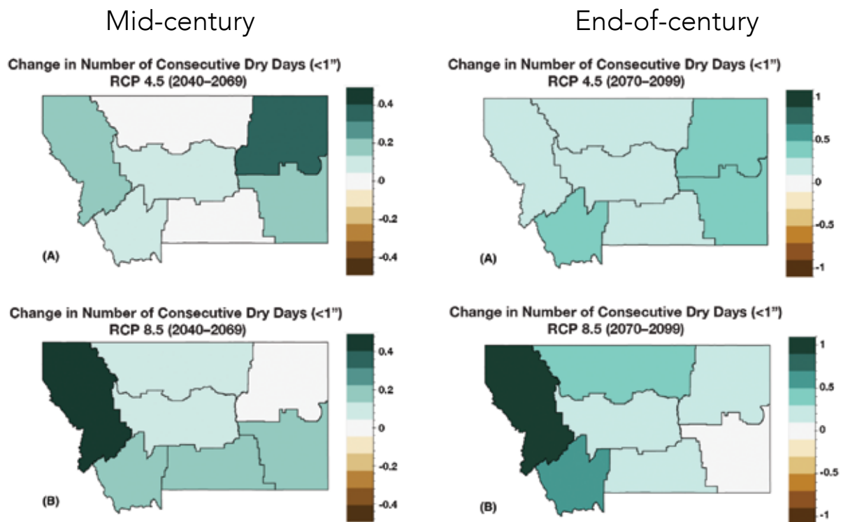
Figure 2-22. The projected change in the number of consecutive dry days (<0.1 inch [0.3 cm] of precipitation) for each climate division in Montana over two periods 2040-2069 and 2070-2099 for (A) stabilization (RCP4.5) and (B) business-as-usual (RCP8.5) emission scenarios.
