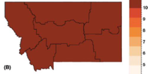
Change in Annual Average Daily Maximum Temperature (°F) RCP 8.5 (2070–2099)
