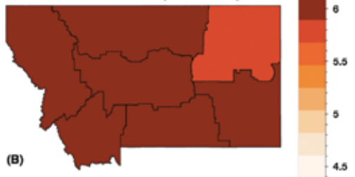
Change in Annual Average Daily Maximum Temperature (°F) RCP 8.5 (2040–2069)
