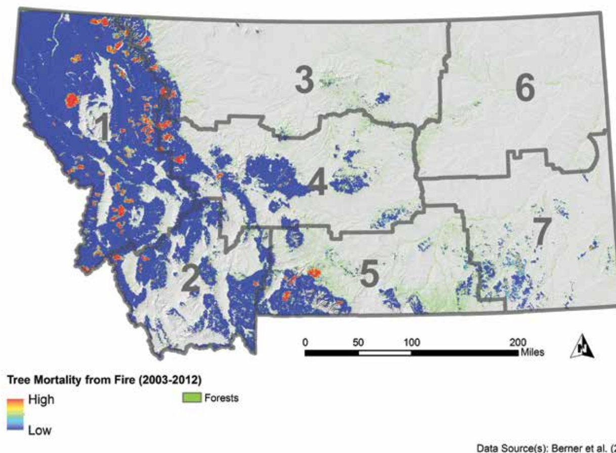
Figure 4-5. Fire severity (measured as total carbon stored in aboveground tissues killed by fire) estimated for 2003-2012, a relatively dry decade. Adapted from Berner et al. (forthcoming).
