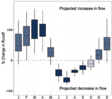
MF Flathead River at West Glacier
