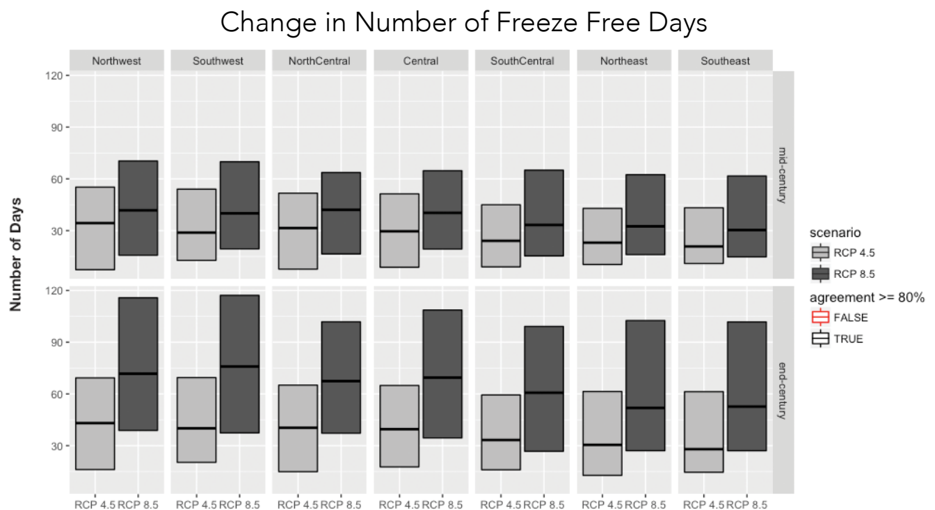
Figure 2-15. Graphs showing the increases in frost-free days/yr projected for each climate division in both stabilization (RCP4.5) and business-as-usual (RCP8.5) emission scenarios. The top row shows mid-century projections (2040-2069) and the bottom row shows end-of-century projections (2070-2099). The outline of each box is determined by model agreement on the sign of the change (positive or negative). A black outline means there is >=80% model agreement and a red outline means that there is <80% model agreement. In this case, all models indicated the direction of the trend of frost-free days at an agreement of greater than 80%.
