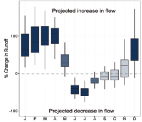
Marias River near Shelby
