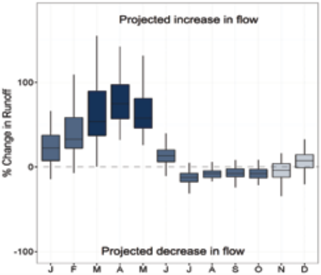
Missouri River at Toston
