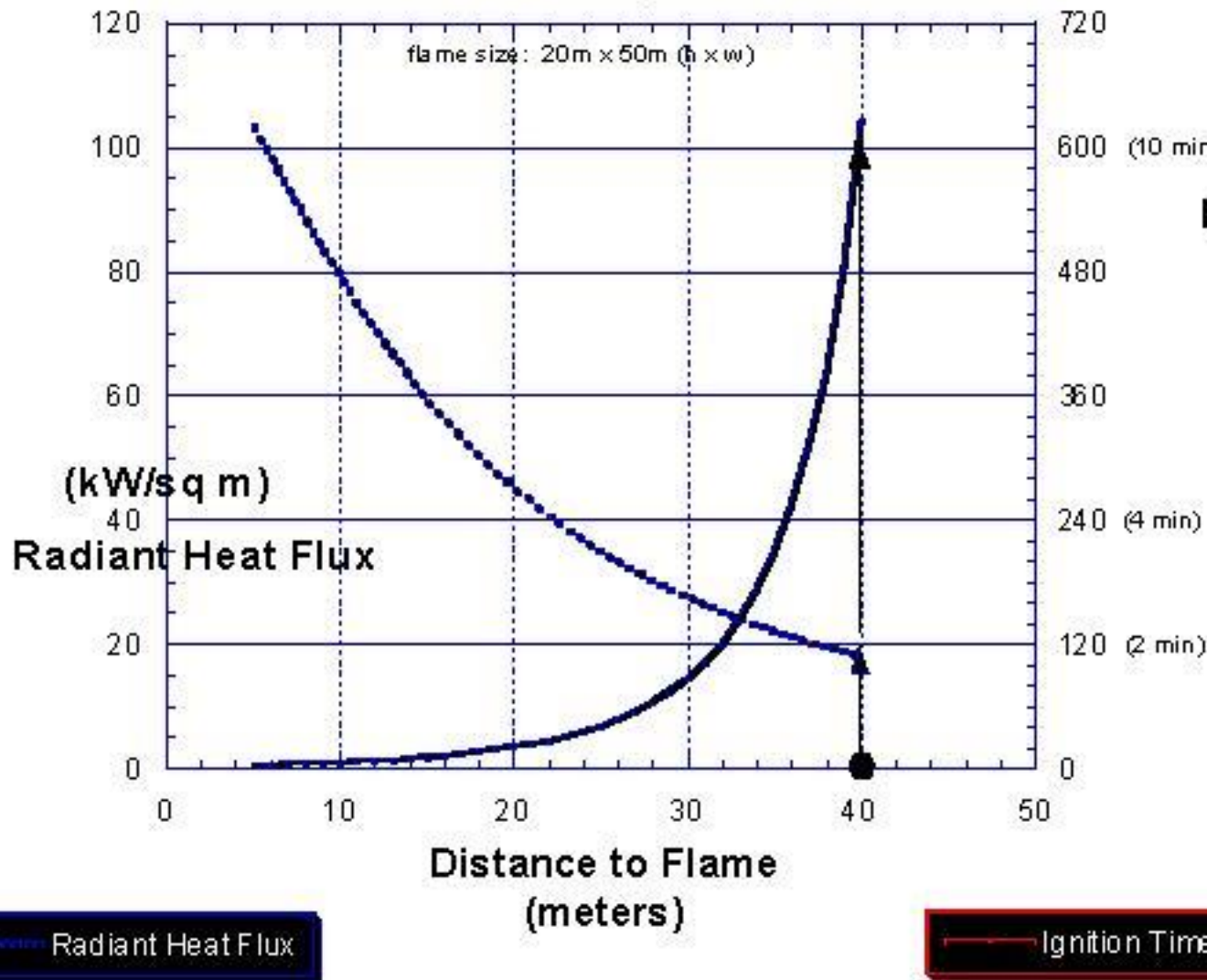
Figure 1-- SIAM calculates the incident radiant heat flux (energy/unit-area/time reaching a surface) and the minimum time for piloted ignition (ignition with a small ignition flame or spark) as a function of distance for the given flame size. The flame is assumed to be a uniform, parallel plane, black body emitter.
